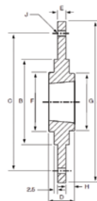
BF Bolt-on-Hub
