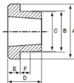
WH Weld-on-Hub
