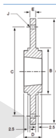
SM Bolt-on-Hub
