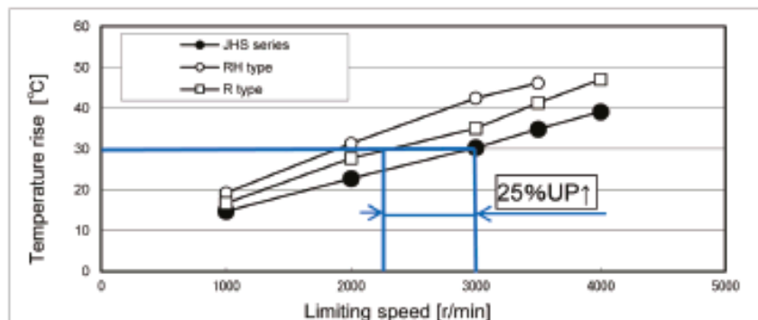
Fig.5: Test results under both radial and axial loads
